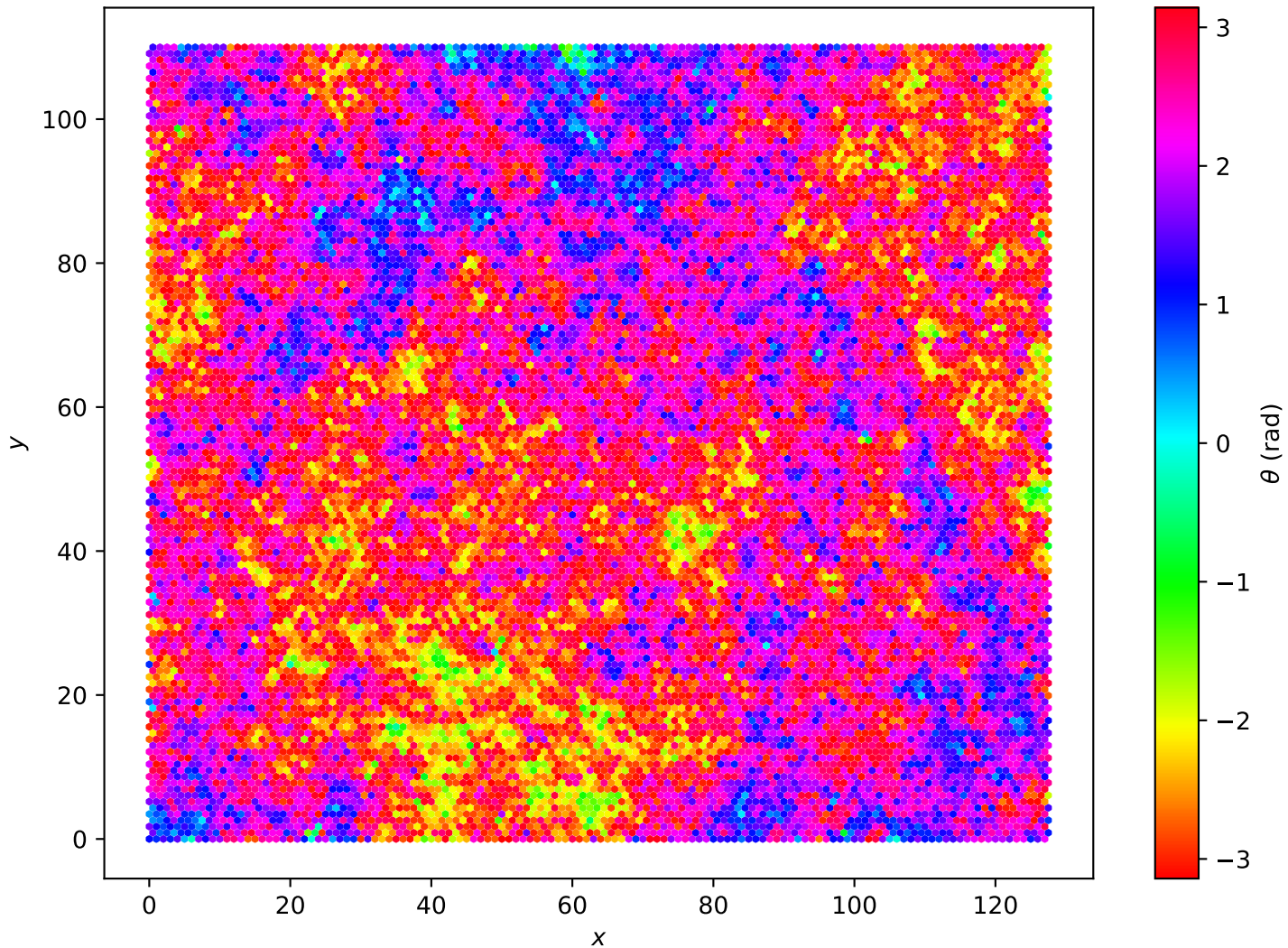
Hexagonal Lattice L=128 , T = 1.10e + 00
