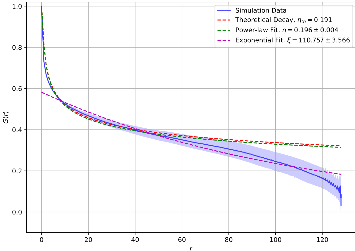
Correlation Function at T = 1.20e + 00 , L = 128
