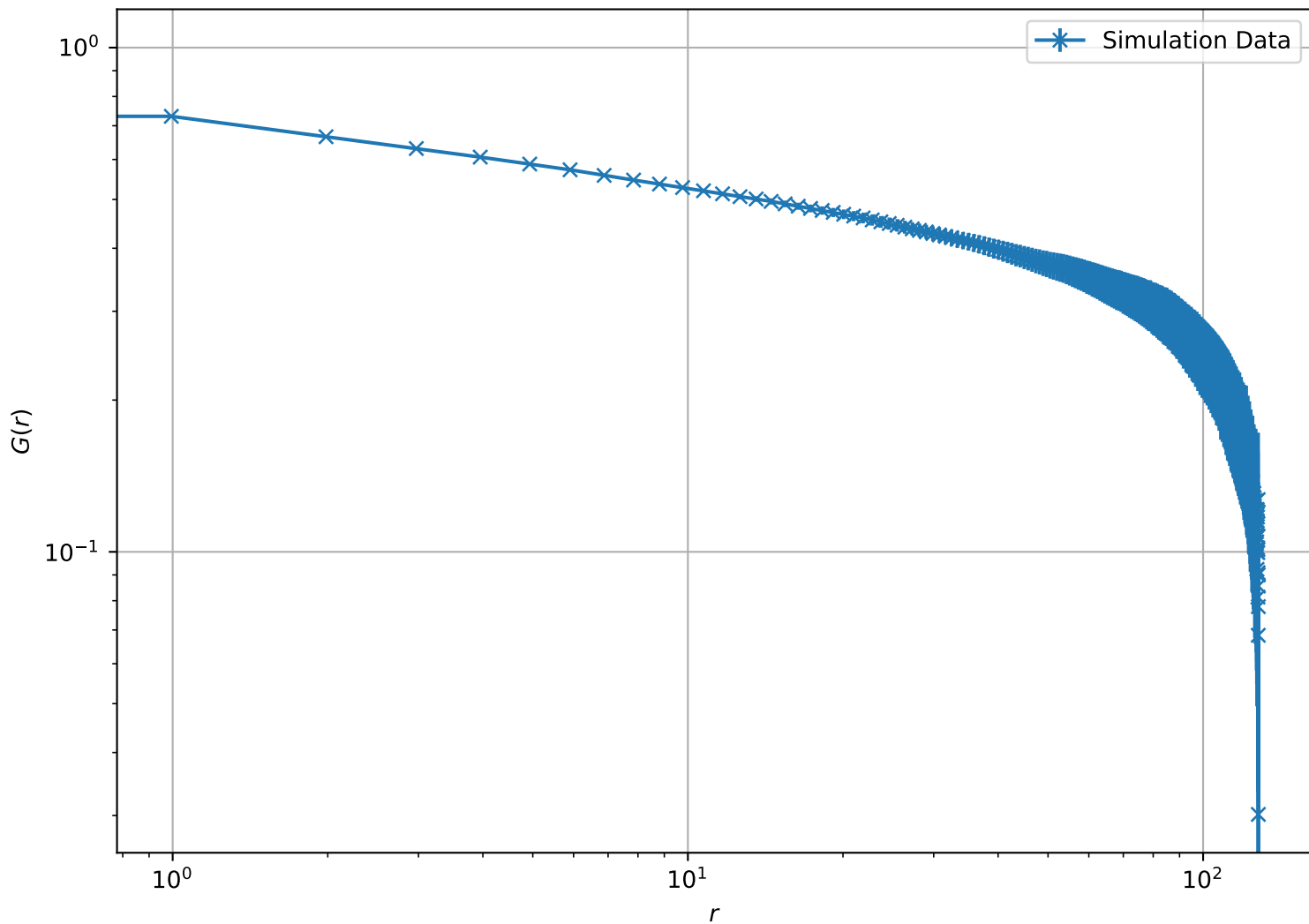
Correlation Function at T = 1.20e + 00 , L = 128 (Log-Log Scale)
