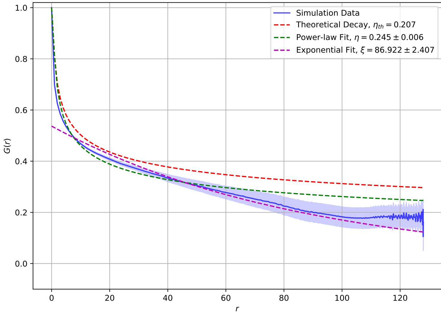
Correlation Function at T = 1.30e + 00 , L = 128
