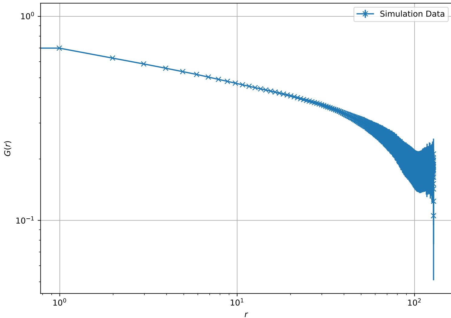
Correlation Function at T = 1.30e + 00 , L = 128 (Log-Log Scale)
