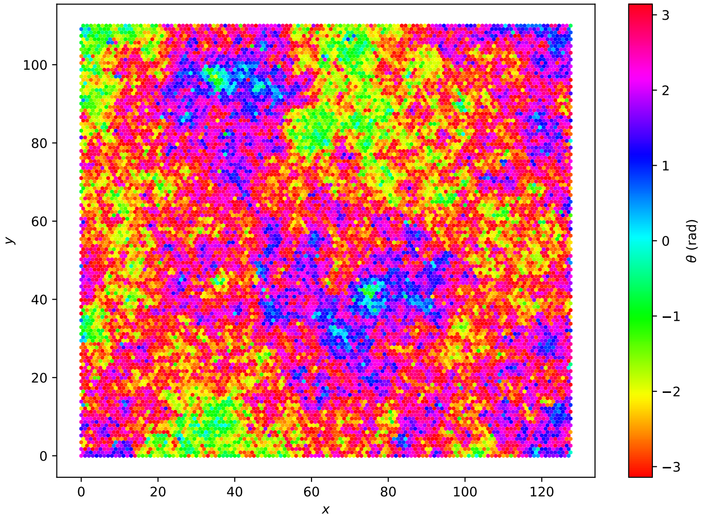
Hexagonal Lattice L=128 , T = 1.30e + 00
