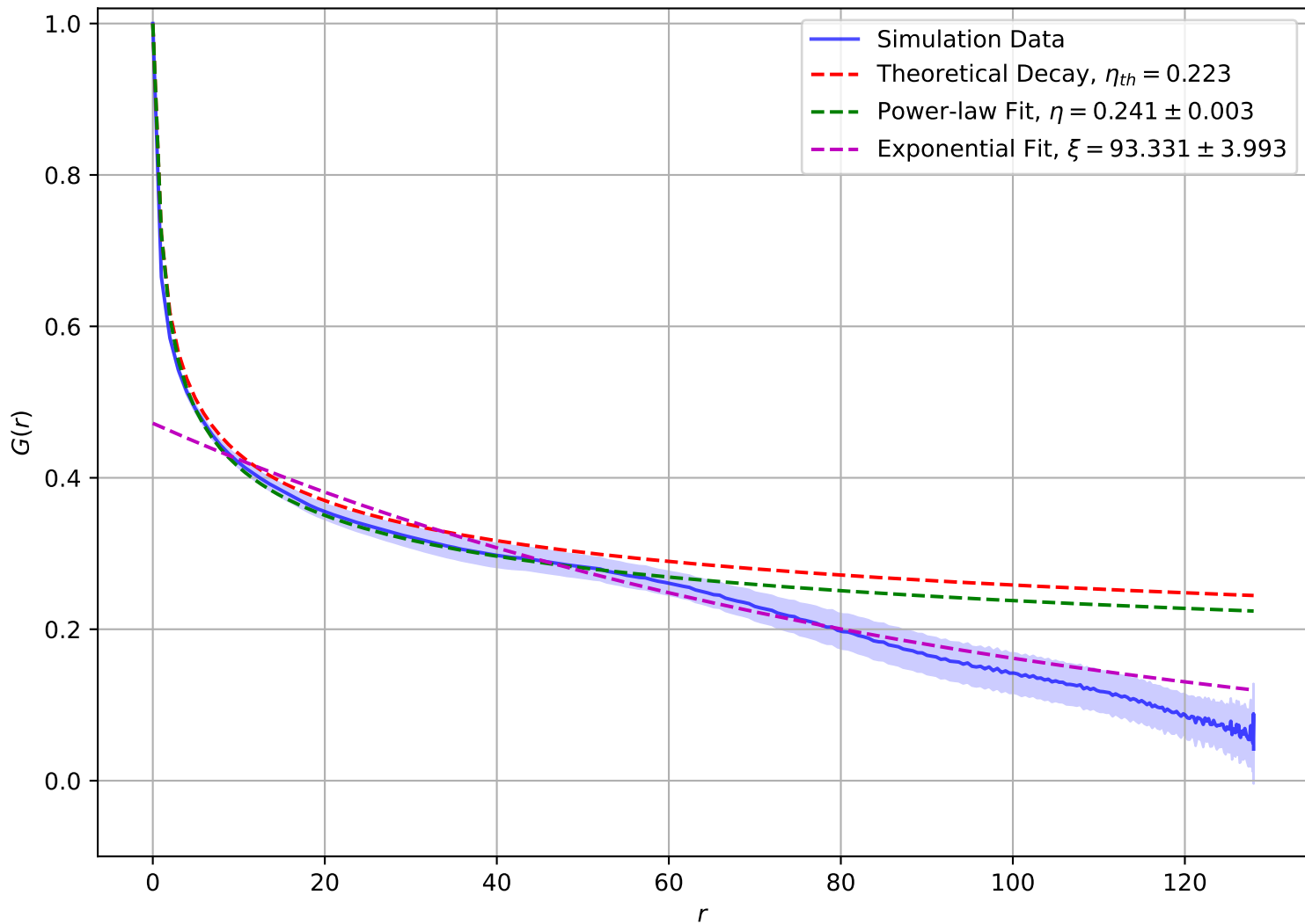
Correlation Function at T = 1.40\text{e} + 00 , L = 128
