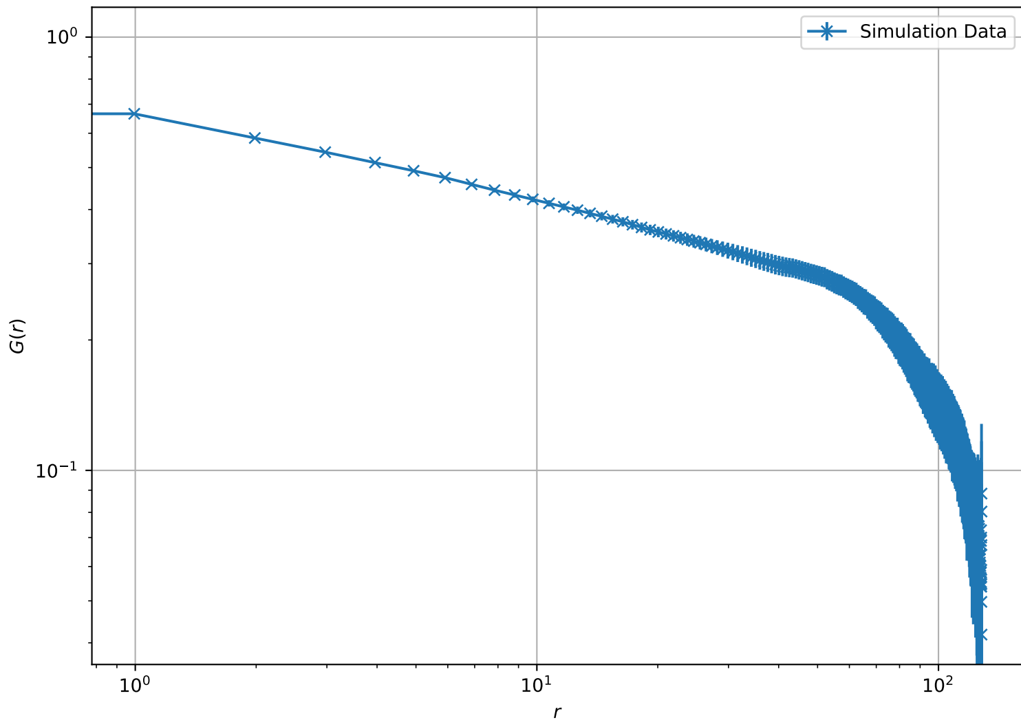
Correlation Function at T = 1.40e + 00 , L = 128 (Log-Log Scale)
