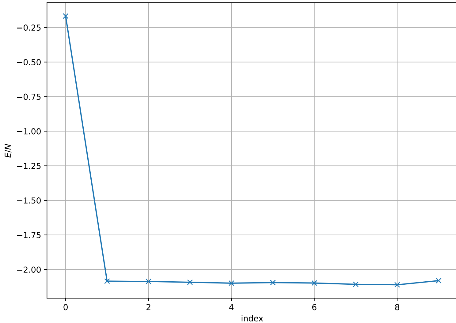
Energy per Site at T = 1.400e + 00 , L = 128
