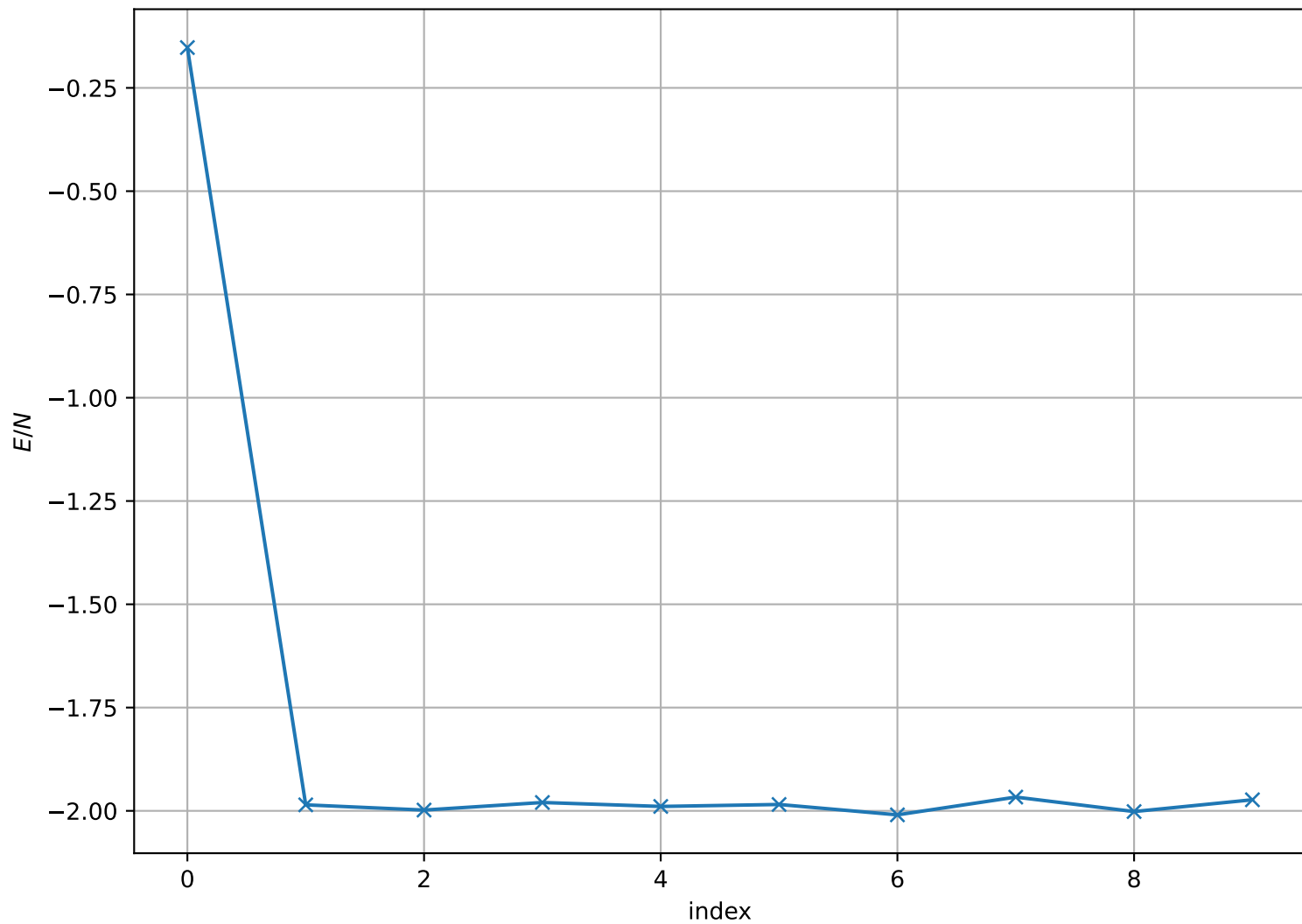
Energy per Site at T = 1.500e + 00 , L = 128
