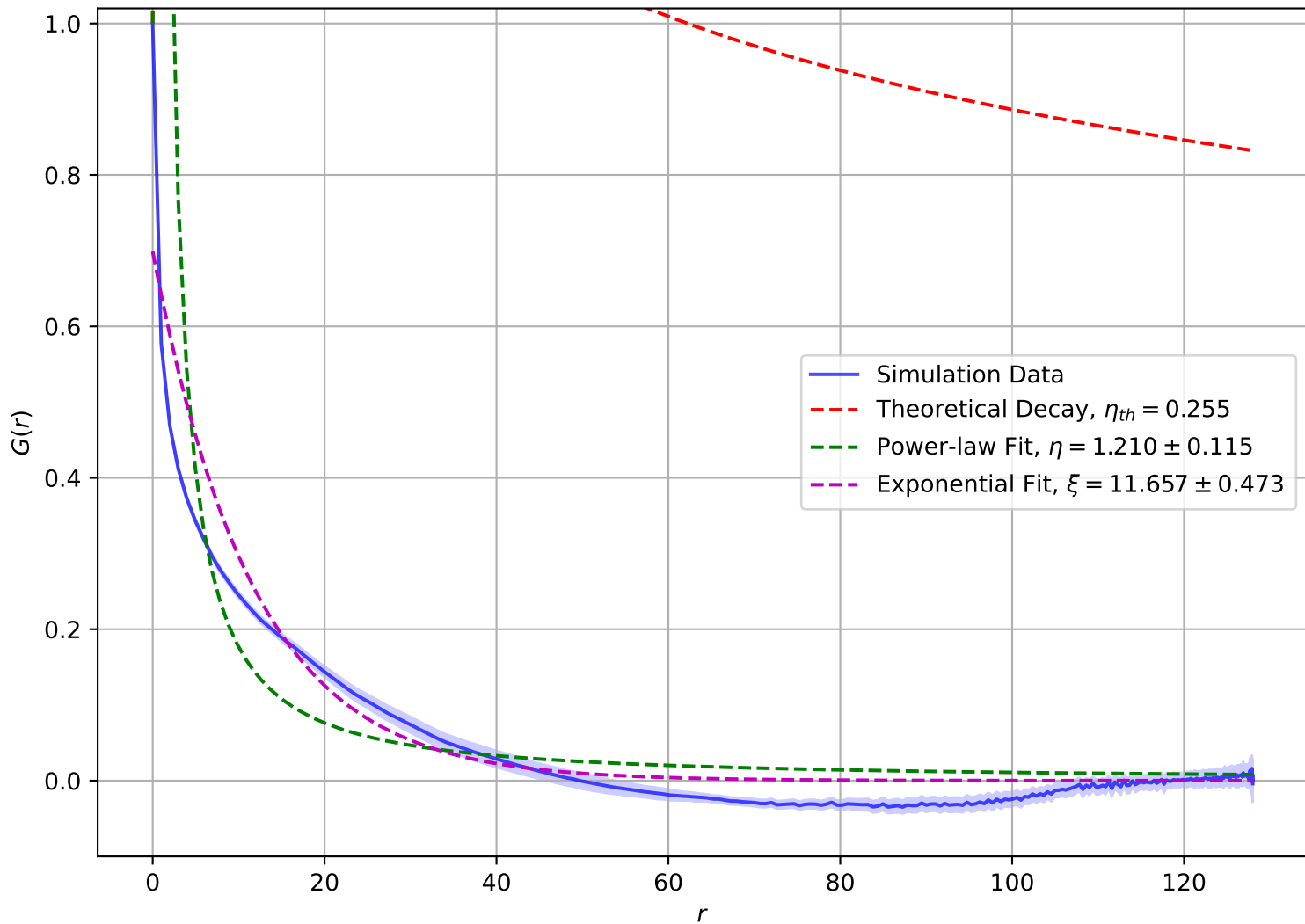
Correlation Function at T = 1.60e + 00 , L = 128
