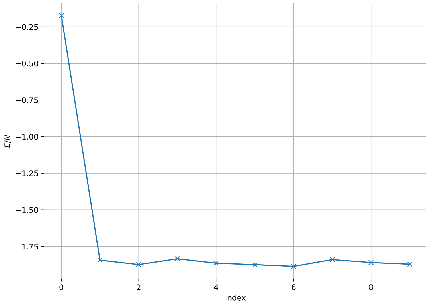
Energy per Site at T = 1.600e + 00 , L = 128
