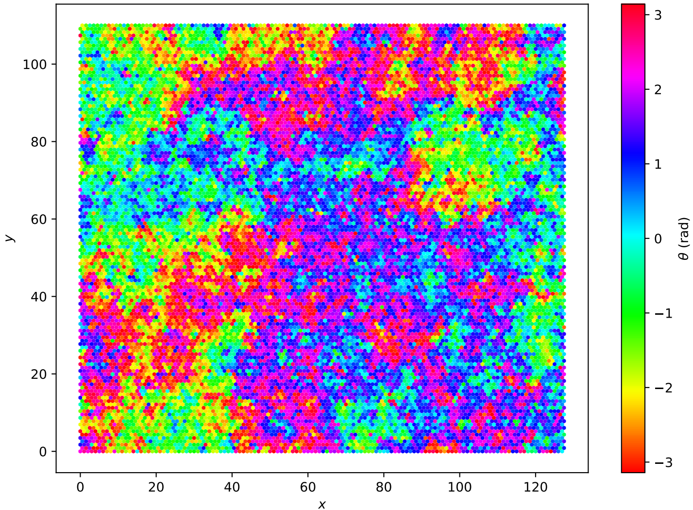
Hexagonal Lattice L=128 , T = 1.60e + 00
