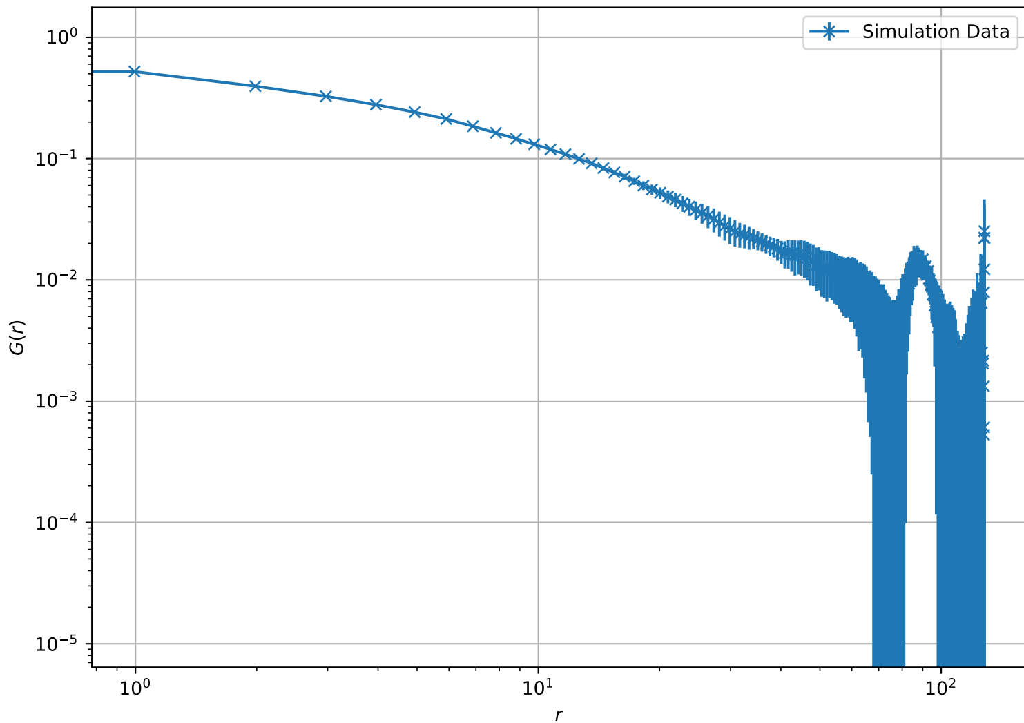
Correlation Function at T = 1.70e + 00 , L = 128 (Log-Log Scale)
