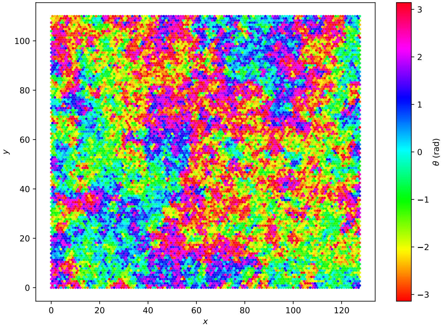
Hexagonal Lattice L=128 , T = 1.70e + 00
