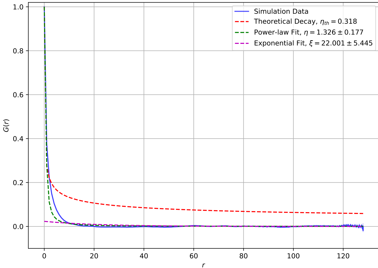
Correlation Function at T = 2.00\text{e} + 00 , L = 128
