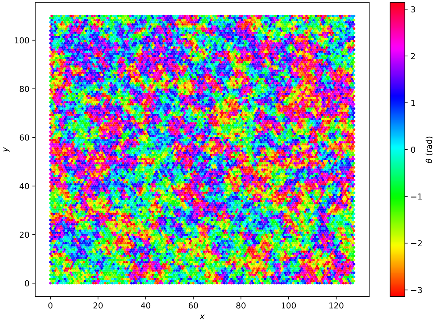
Hexagonal Lattice L=128 , T = 2.00e + 00
