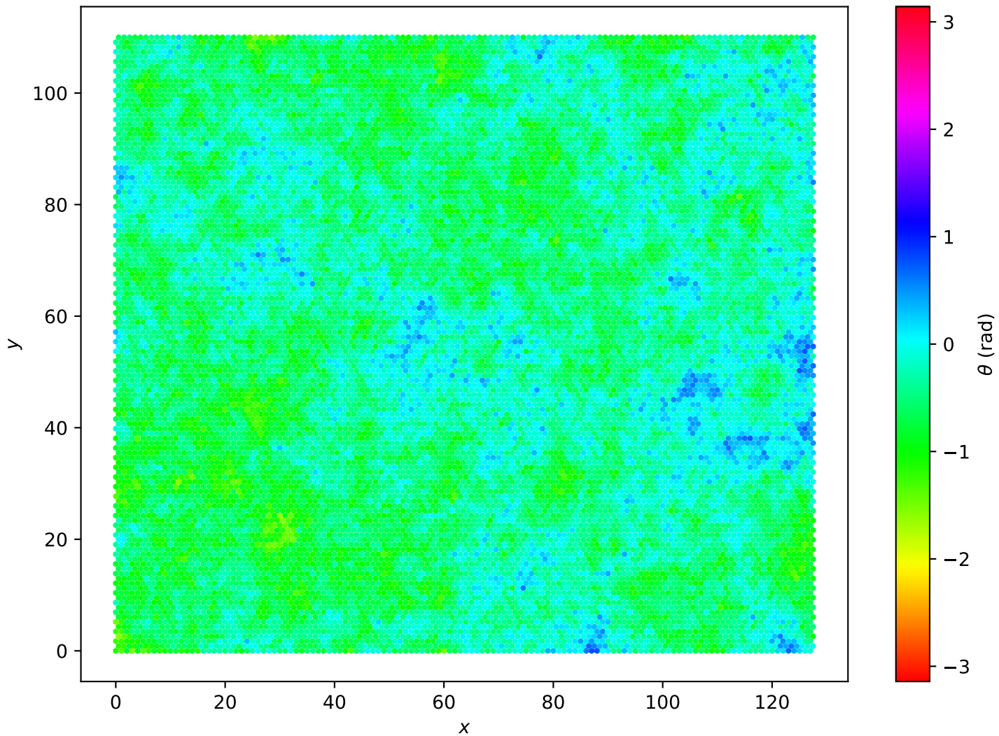
Hexagonal Lattice L=128 , T = 2.00e - 01
