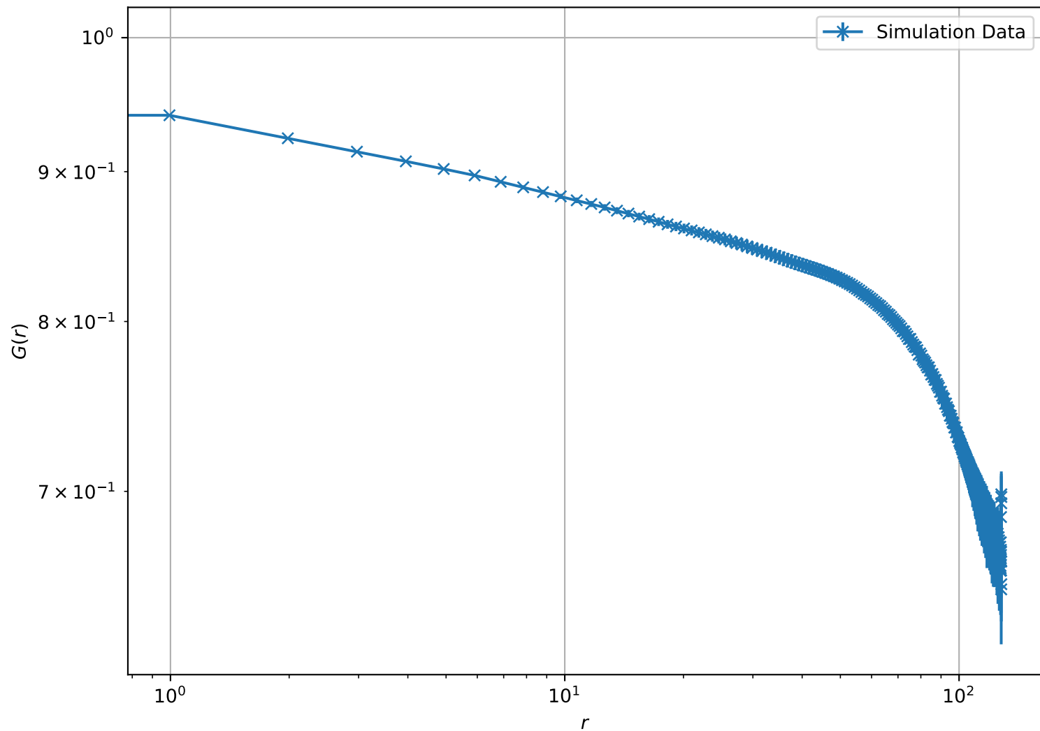
Correlation Function at T = 3.00e - 01 , L = 128 (Log-Log Scale)
