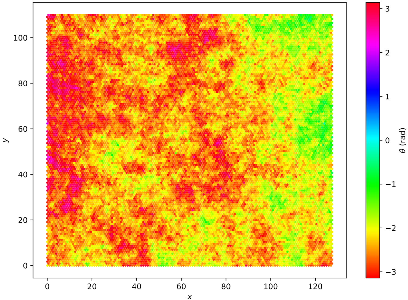
Hexagonal Lattice L=128 , T = 3.00e - 01
