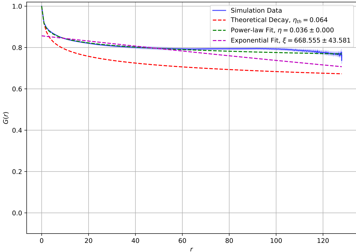
Correlation Function at T = 4.00\text{e} - 01 , L = 128
