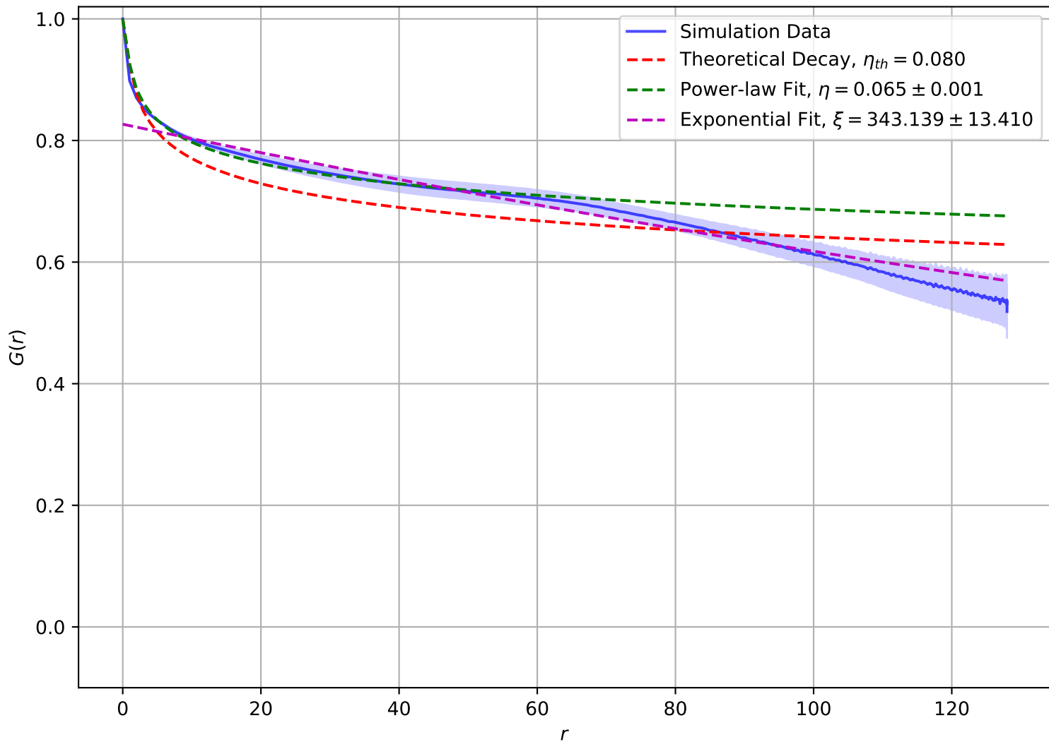
Correlation Function at T = 5.00\text{e} - 01 , L = 128
