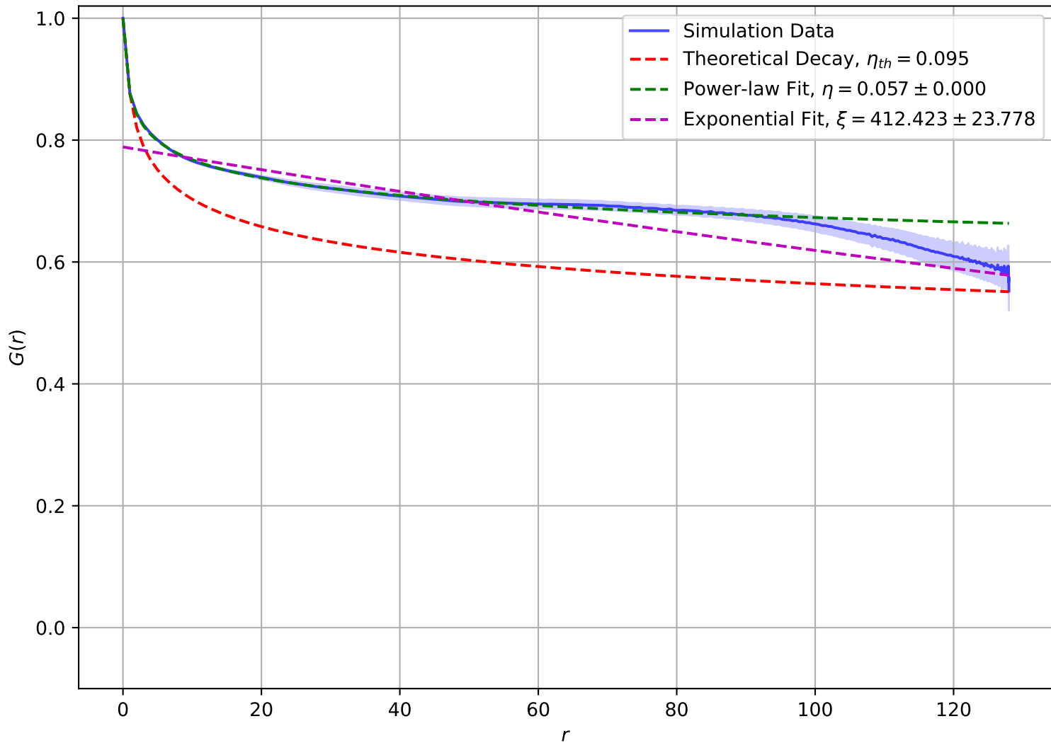
Correlation Function at T = 6.00e - 01 , L = 128
