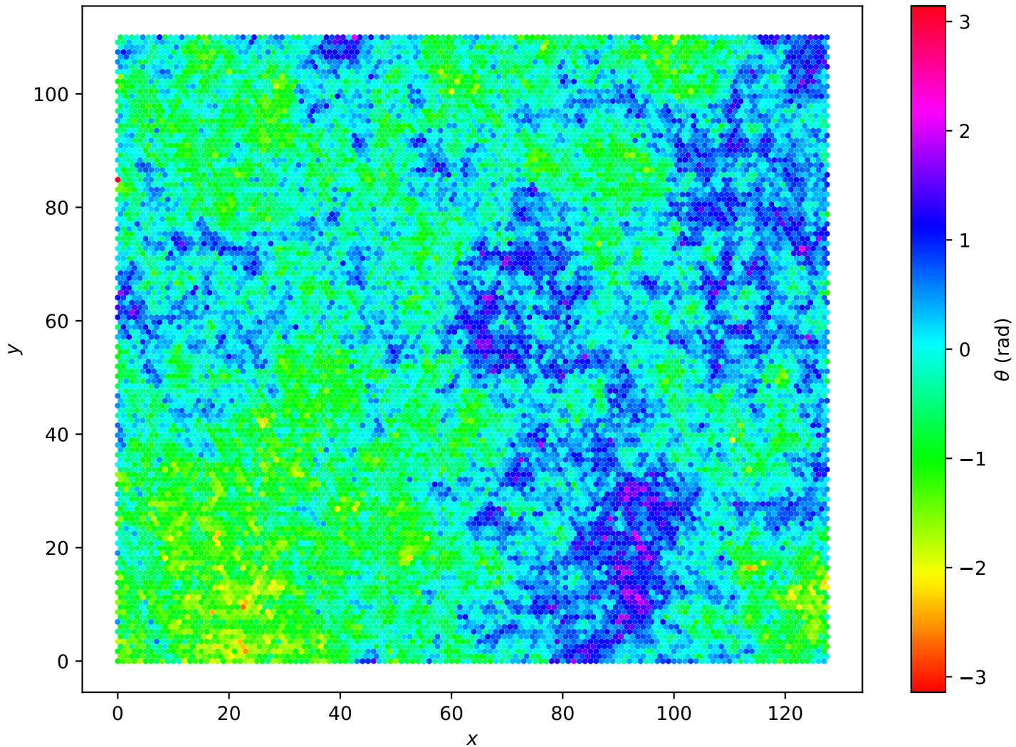
Hexagonal Lattice L=128 , T = 6.00e - 01
