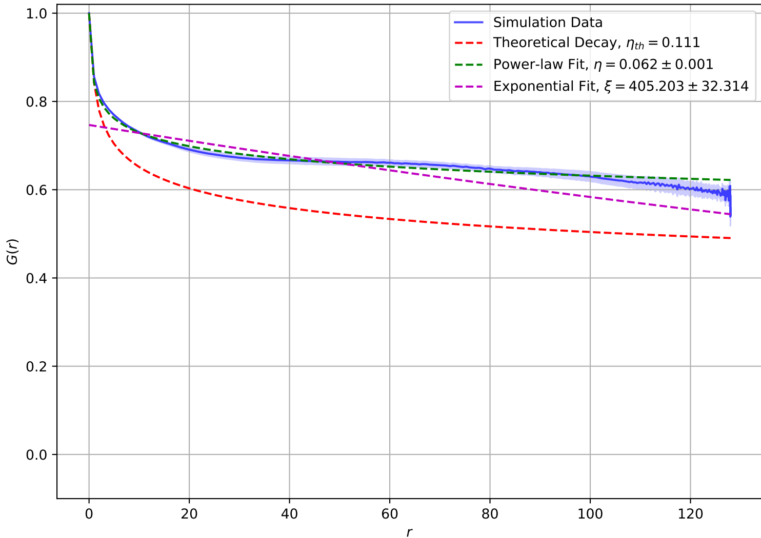
Correlation Function at T = 7.00e - 01 , L = 128
