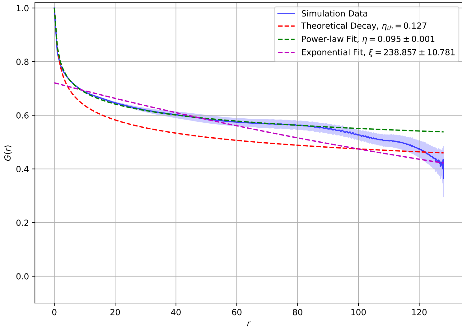
Correlation Function at T = 8.00e - 01 , L = 128
