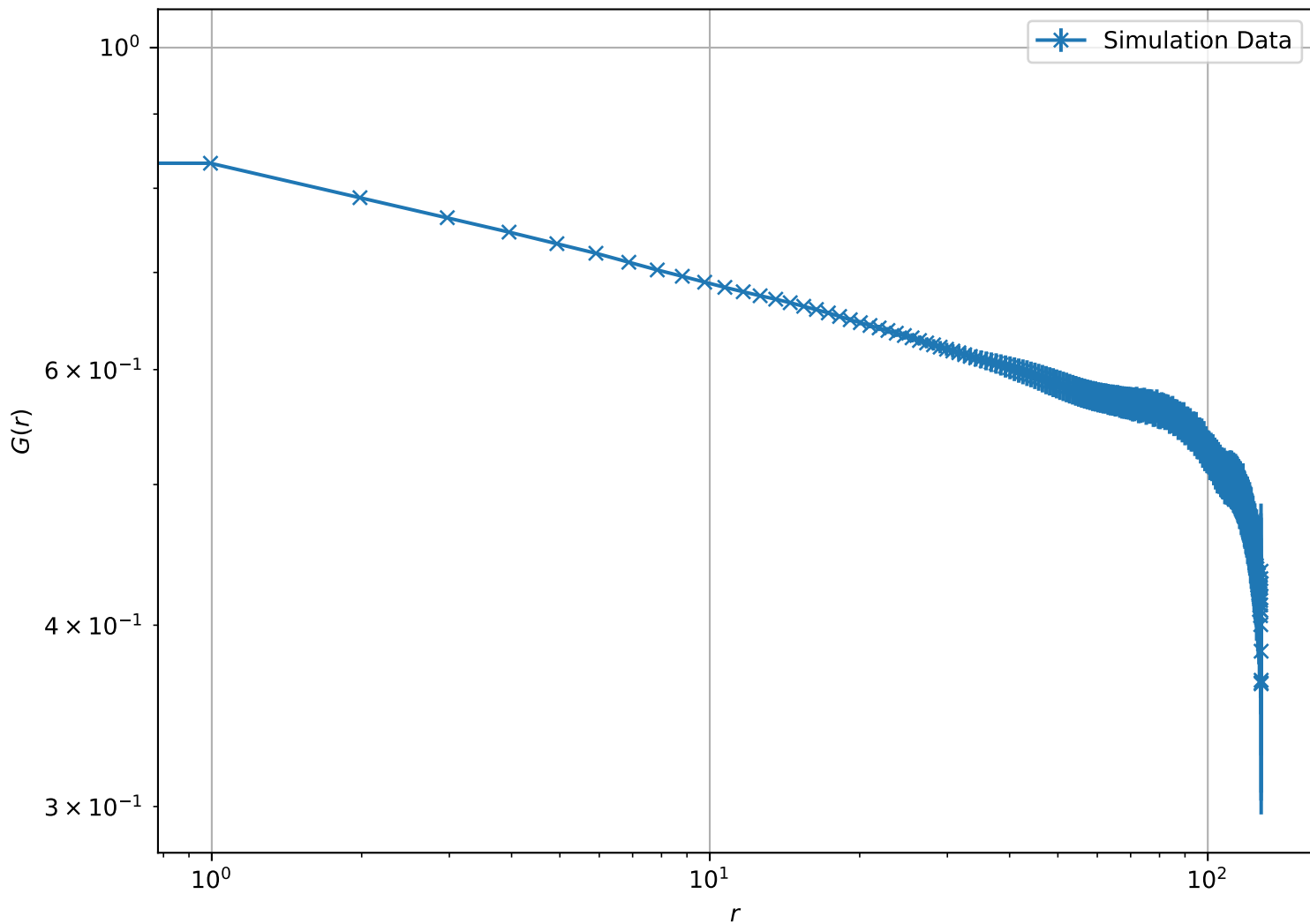
Correlation Function at T = 8.00e - 01 , L = 128 (Log-Log Scale)
