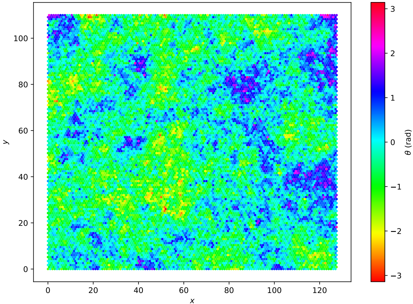
Hexagonal Lattice L=128 , T = 9.00e - 01
