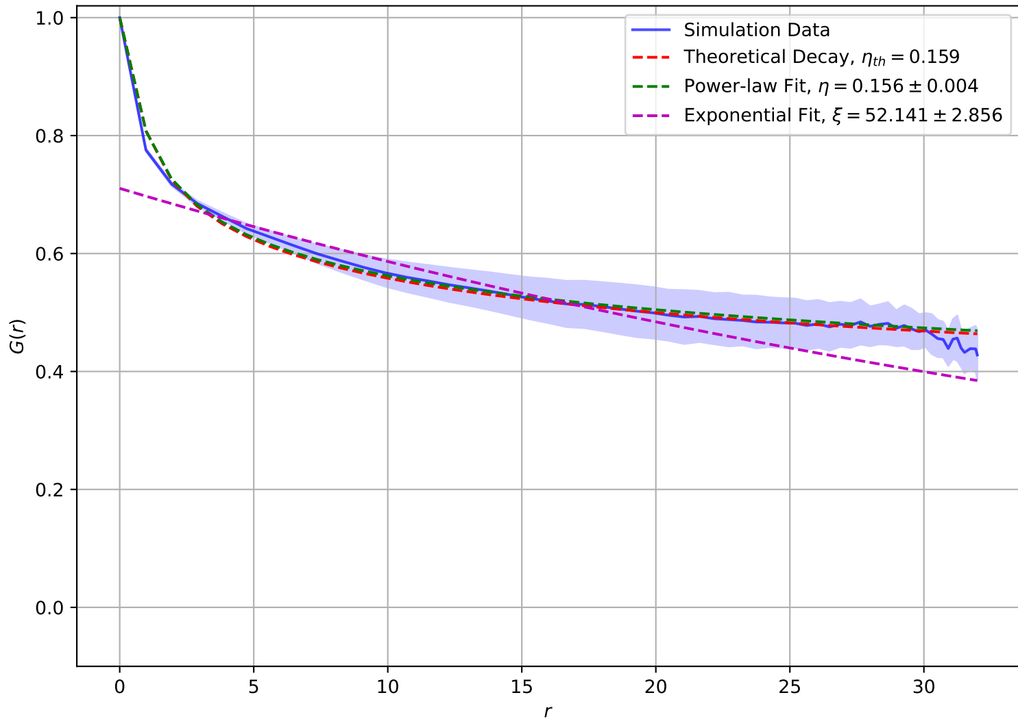
Correlation Function at T = 1.00e + 00 , L = 32
