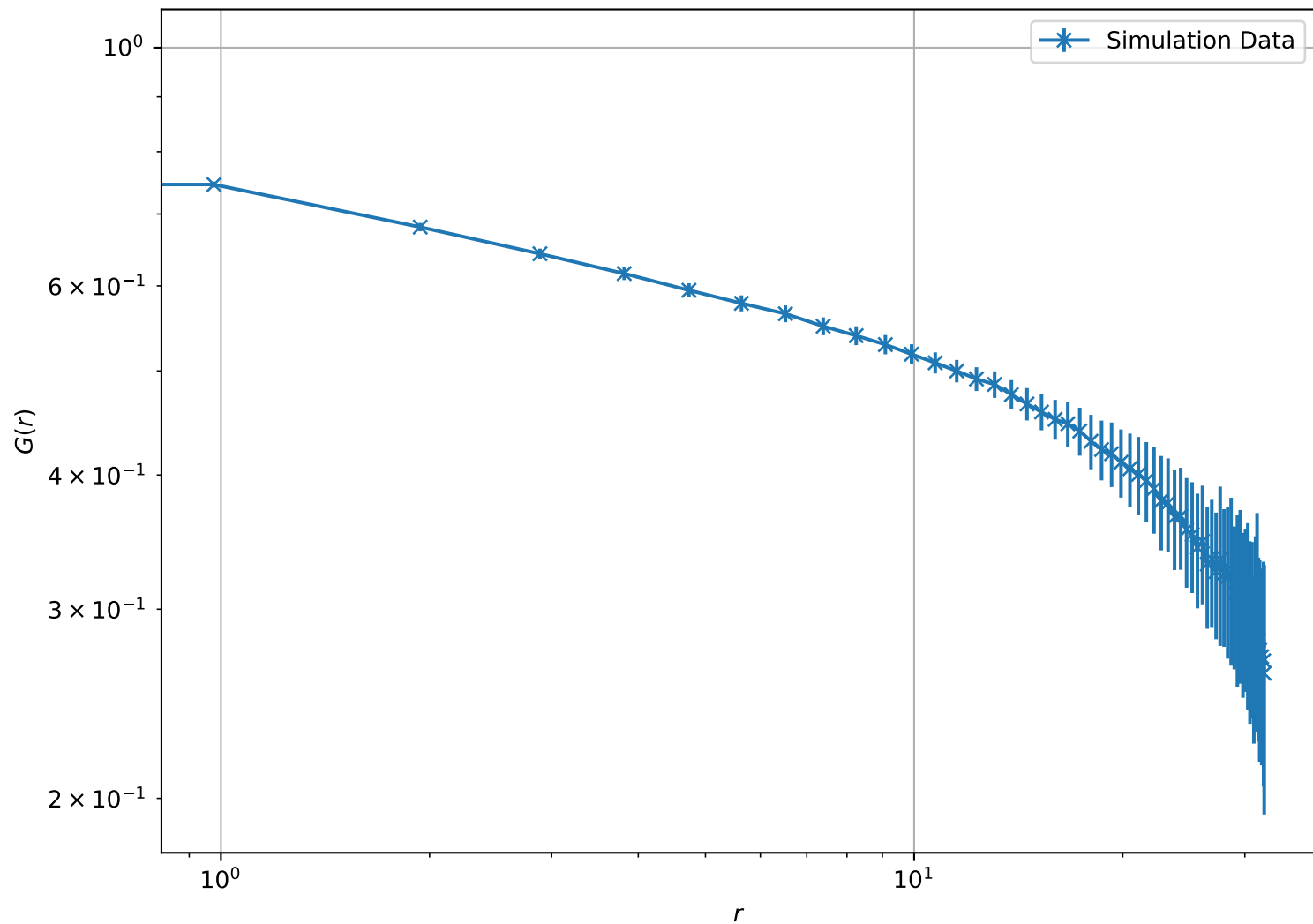
Correlation Function at T = 1.10e + 00 , L = 32 (Log-Log Scale)
