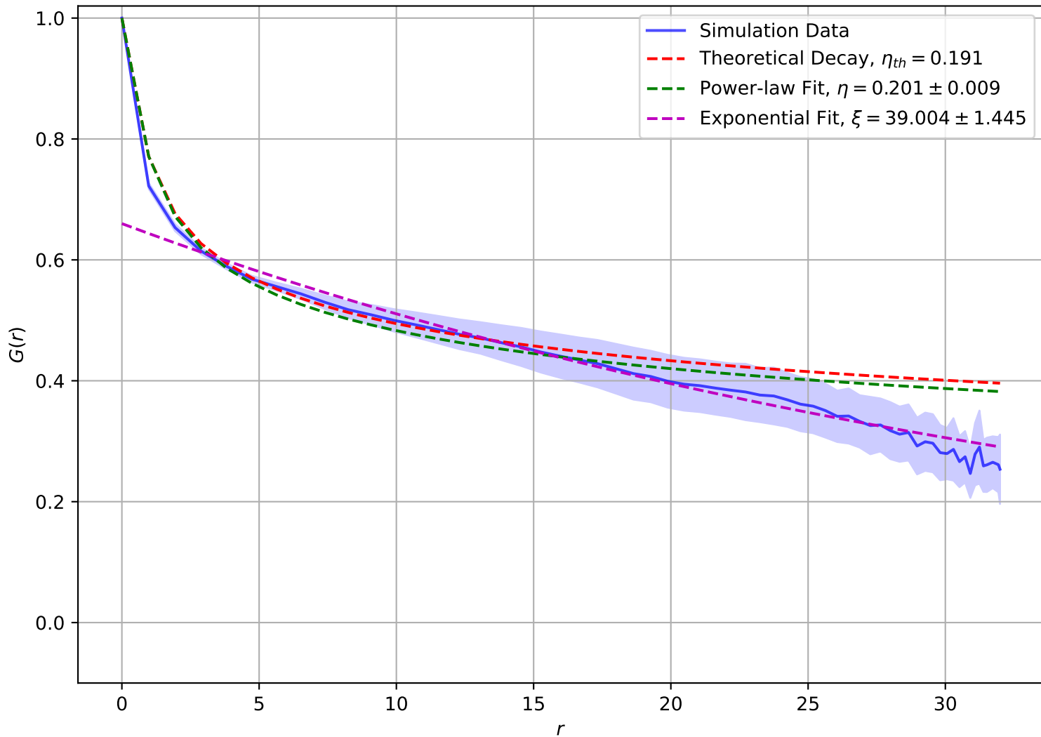
Correlation Function at T = 1.20e + 00 , L = 32
