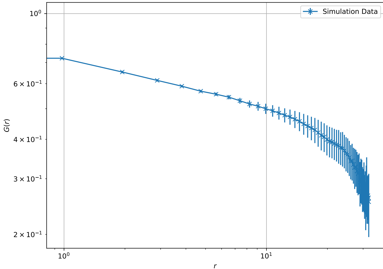
Correlation Function at T = 1.20e + 00 , L = 32 (Log-Log Scale)
