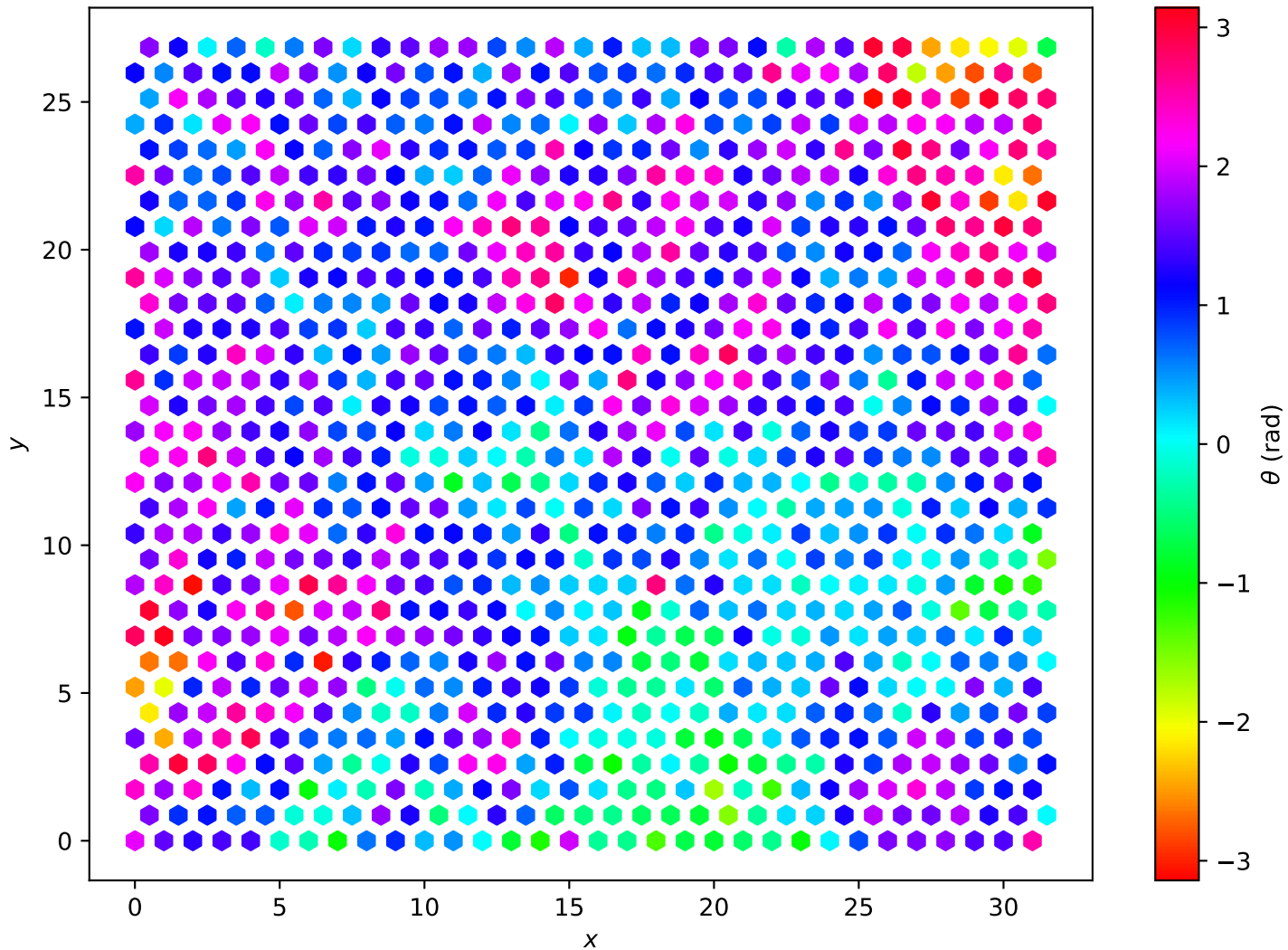
Hexagonal Lattice L=32 , T = 1.20e + 00
