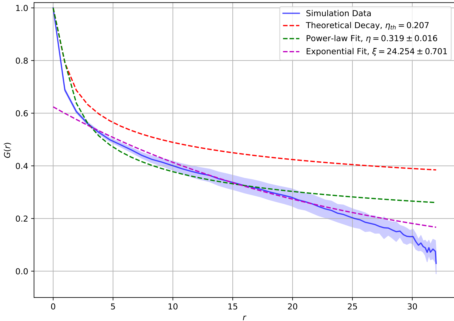
Correlation Function at T = 1.30e + 00 , L = 32
