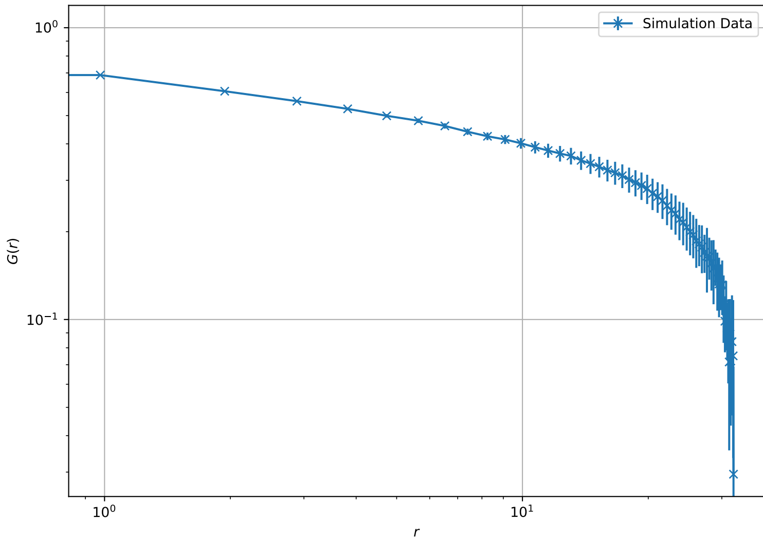
Correlation Function at T = 1.30e + 00 , L = 32 (Log-Log Scale)
