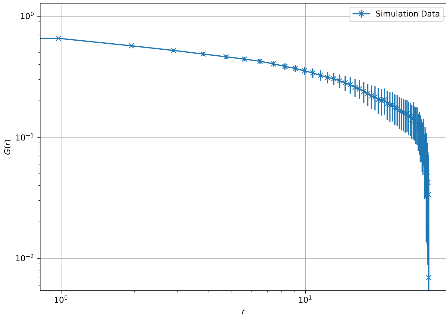
Correlation Function at T = 1.40e + 00 , L = 32 (Log-Log Scale)
