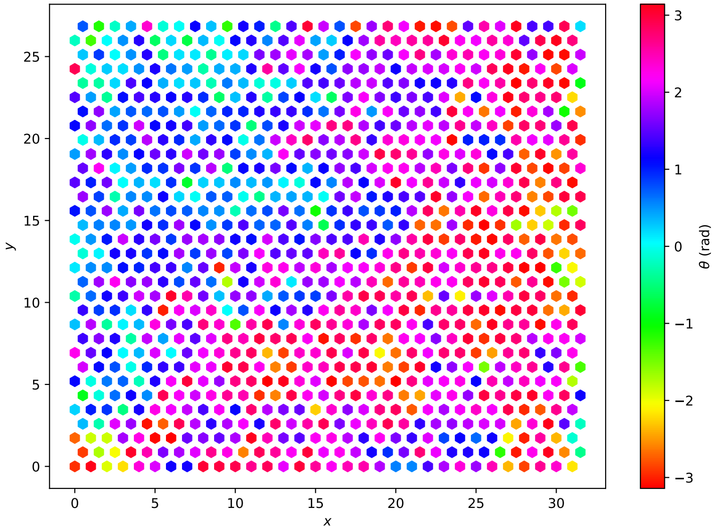
Hexagonal Lattice L=32 , T = 1.40e + 00
