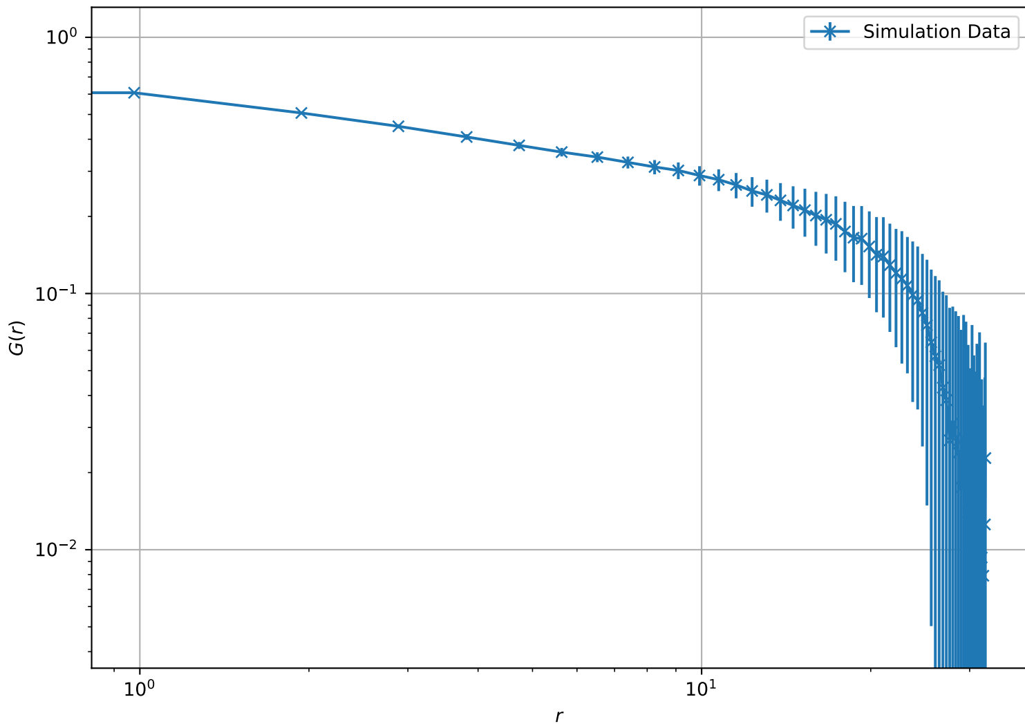
Correlation Function at T = 1.50e + 00 , L = 32 (Log-Log Scale)
