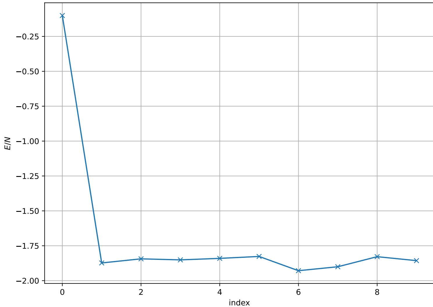
Energy per Site at T = 1.500e + 00 , L = 32
