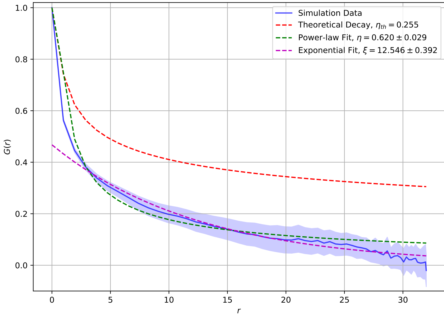
Correlation Function at T = 1.60e + 00 , L = 32
