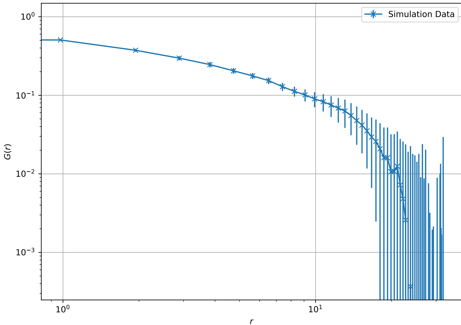
Correlation Function at T = 1.70e + 00 , L = 32 (Log-Log Scale)
