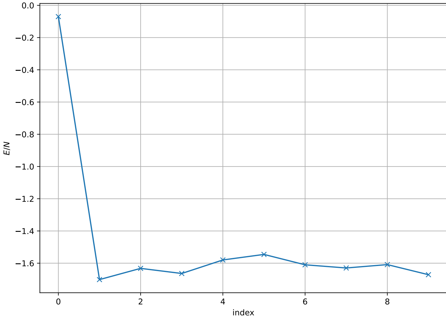
Energy per Site at T = 1.700e + 00 , L = 32
