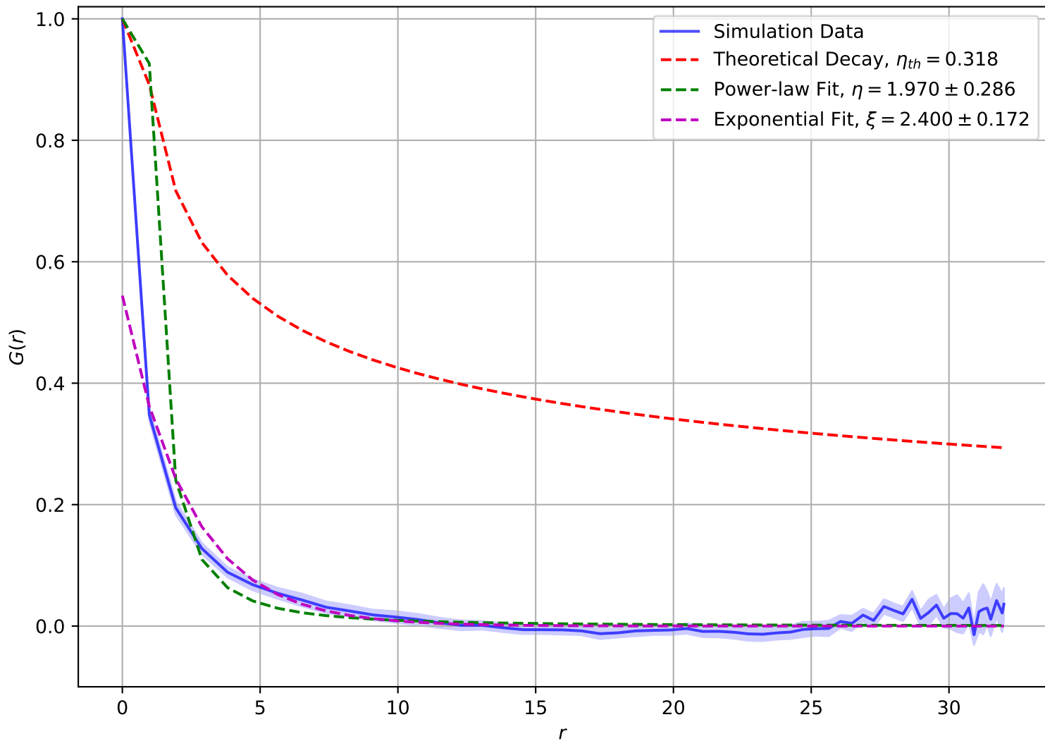
Correlation Function at T = 2.00\text{e} + 00 , L = 32
