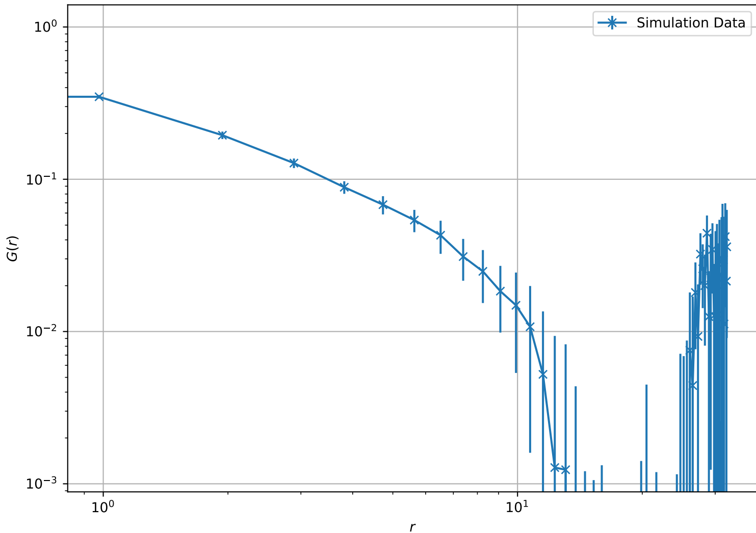
Correlation Function at T = 2.00e + 00 , L = 32 (Log-Log Scale)
