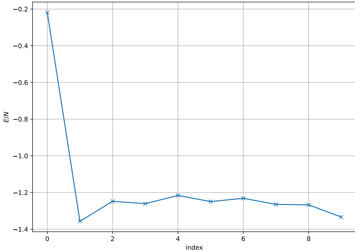
Energy per Site at T = 2.000e + 00 , L = 32
