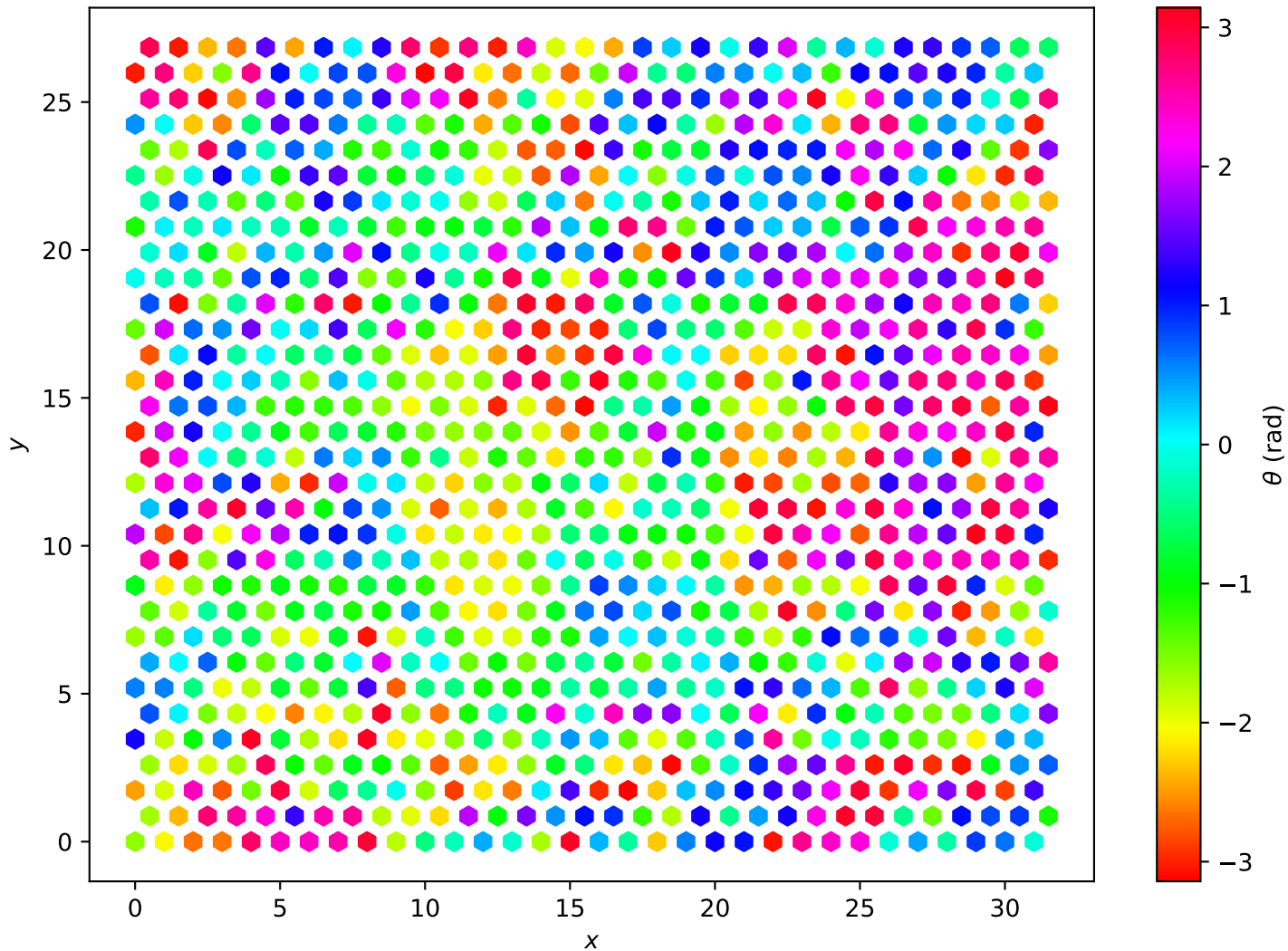
Hexagonal Lattice L=32 , T = 2.00e + 00
