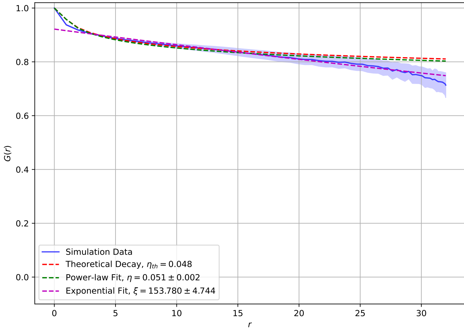
Correlation Function at T = 3.00e - 01 , L = 32
