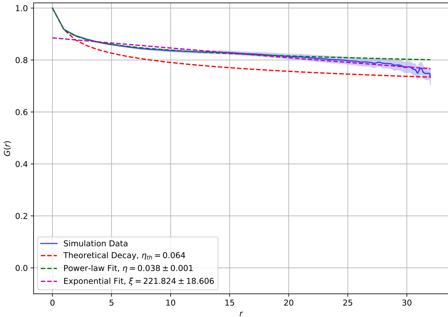
Correlation Function at T = 4.00e - 01 , L = 32
