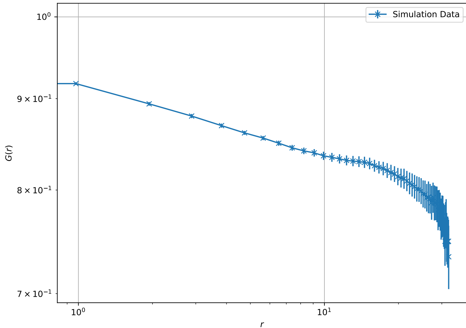
Correlation Function at T = 4.00e - 01 , L = 32 (Log-Log Scale)
