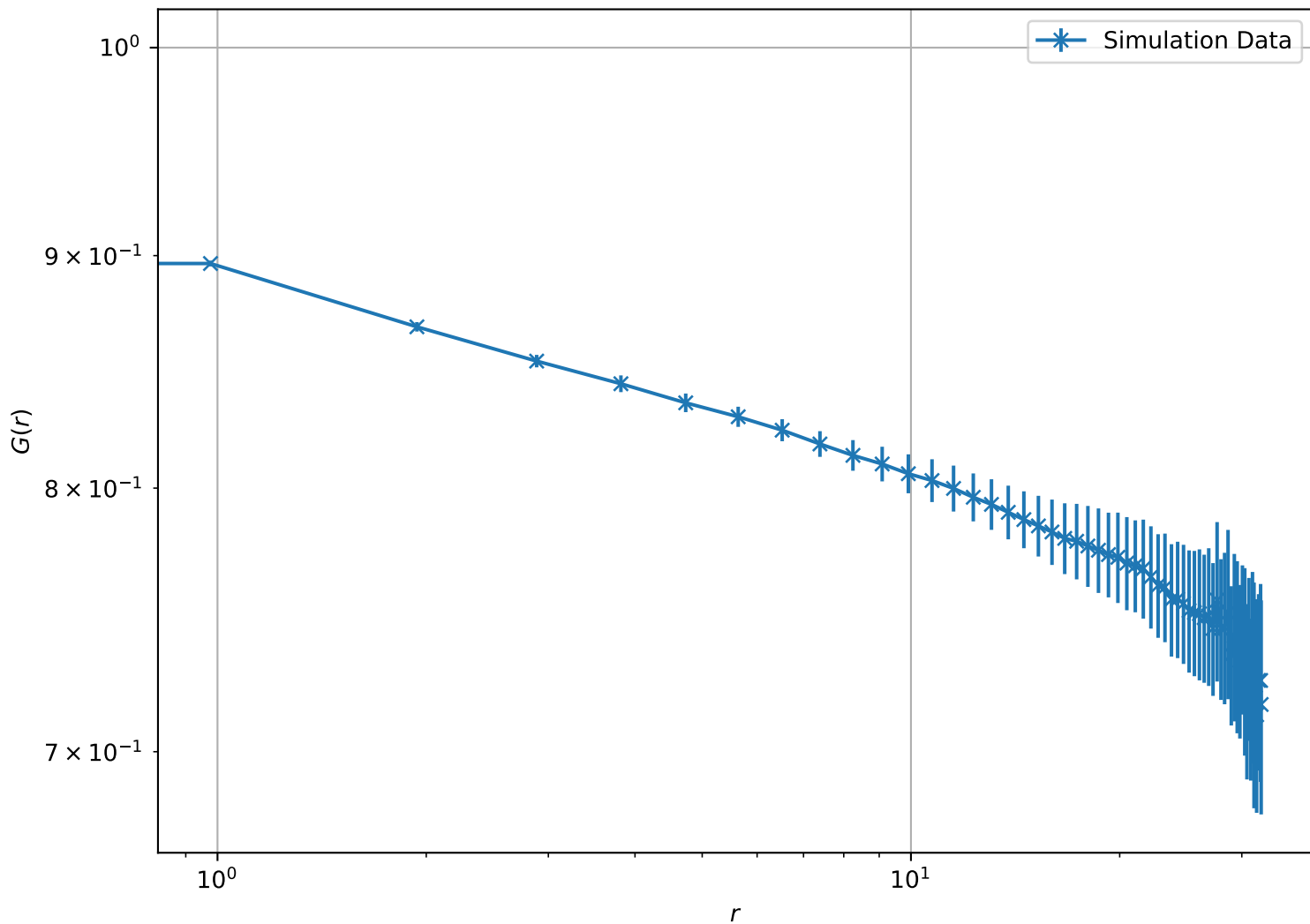
Correlation Function at T = 5.00e - 01 , L = 32 (Log-Log Scale)
